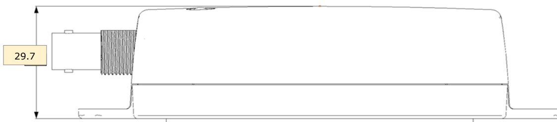
Figure 7 - Modbus pH Sensor Adapter Dimension – Side View
