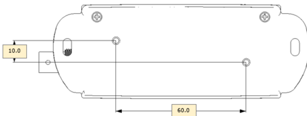
Figure 8 - Modbus pH Sensor Adapter Dimension – Bottom View
