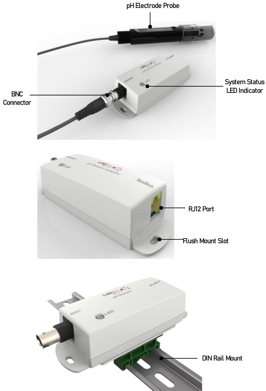
Figure 1 - Modbus pH Sensor Adapter Hardware Features
