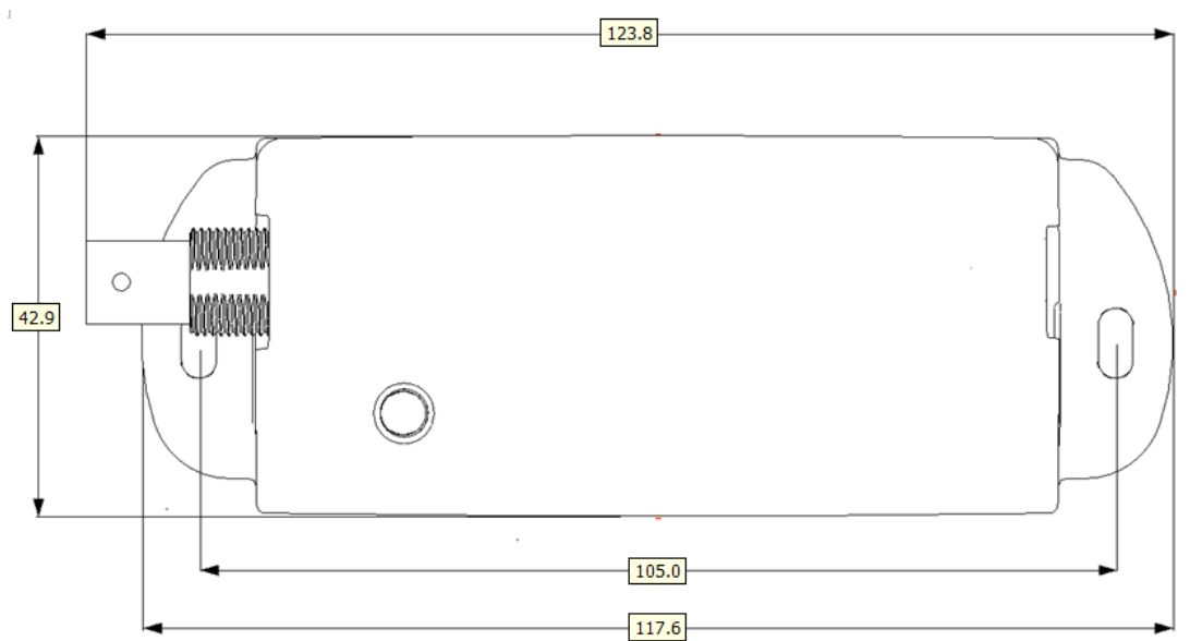
Figure 6 - Modbus pH Sensor Adapter Dimension – Top View
