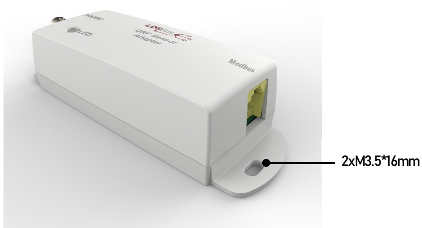
Figure 4 - Modbus ORP Sensor Adapter Flush Mount
