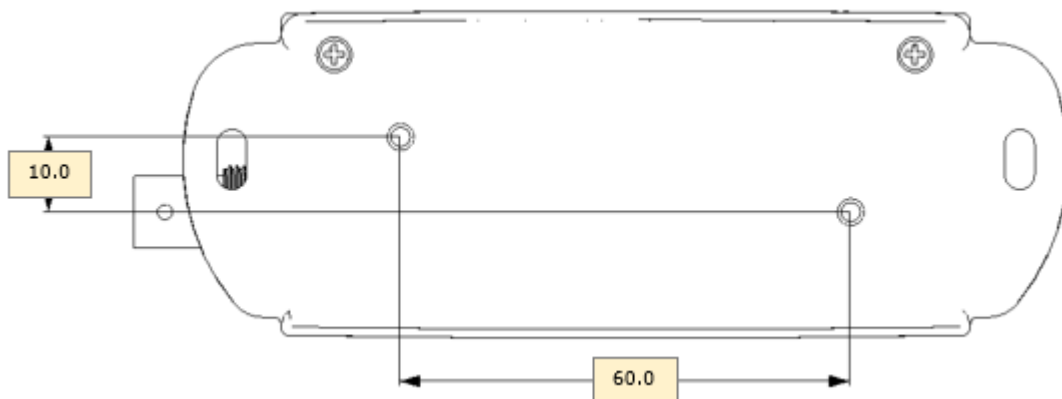
Figure 8 - Modbus ORP Sensor Adapter Dimension – Bottom View
