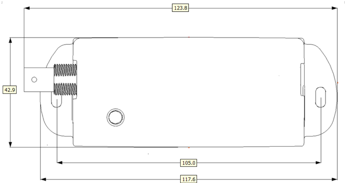
Figure 6 - Modbus ORP Sensor Adapter Dimension – Top View
