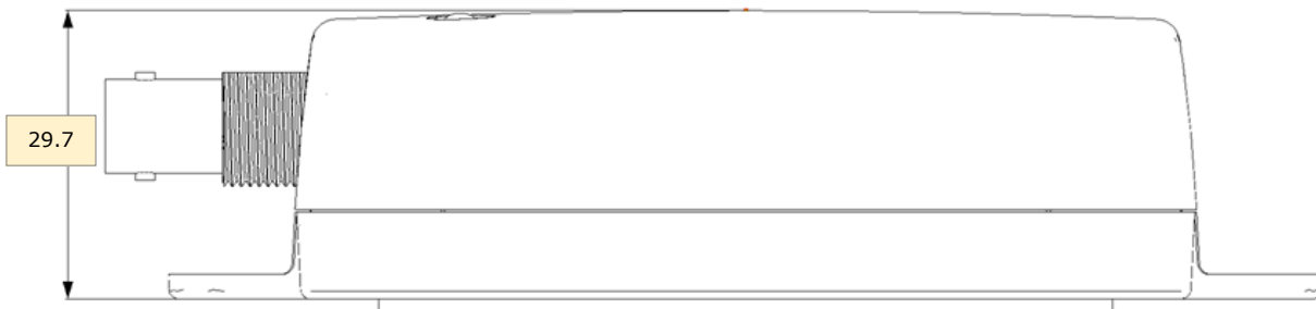
Figure 7 - Modbus ORP Sensor Adapter Dimension – Side View
