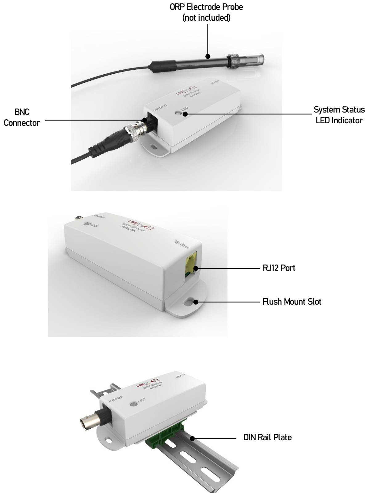
Figure 1 - Modbus ORP Sensor Adapter Hardware Features
