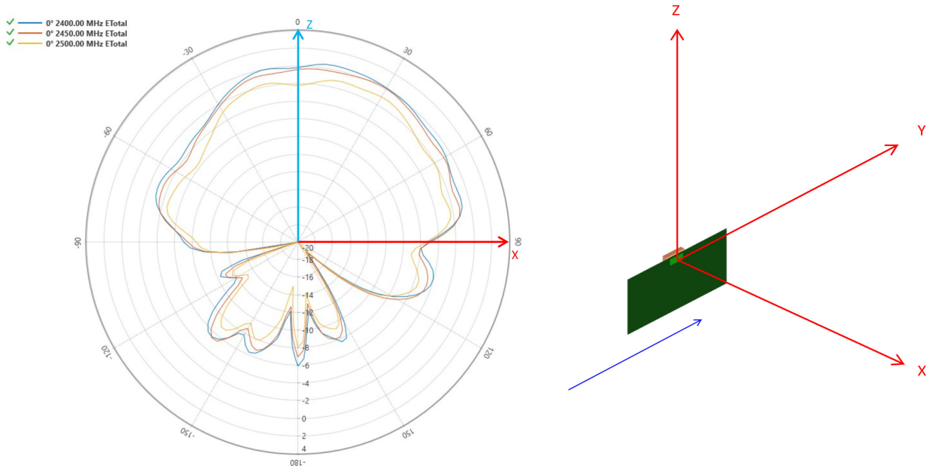
Figure 4.3. BGM270S Typical 2D Antenna Radiation Patterns on 55 mm x 30 mm board - \Phi = 0^\circ Gain (dBi)
