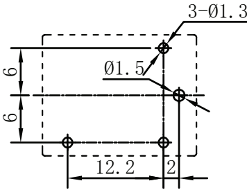
Recommended PCB Layout Bottom View
