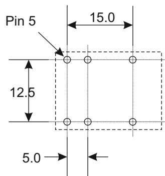
PCB Top Side View
