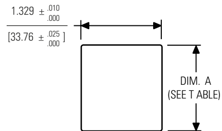
Mounting Detail
