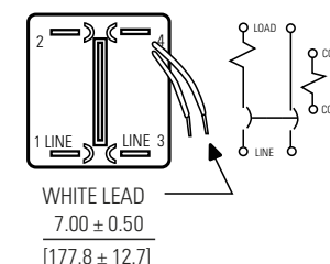
Two Pole ( 1 pole relay )
