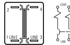
Two Pole ( 1 pole shunt )
