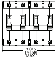
Panel Mounting Detail
