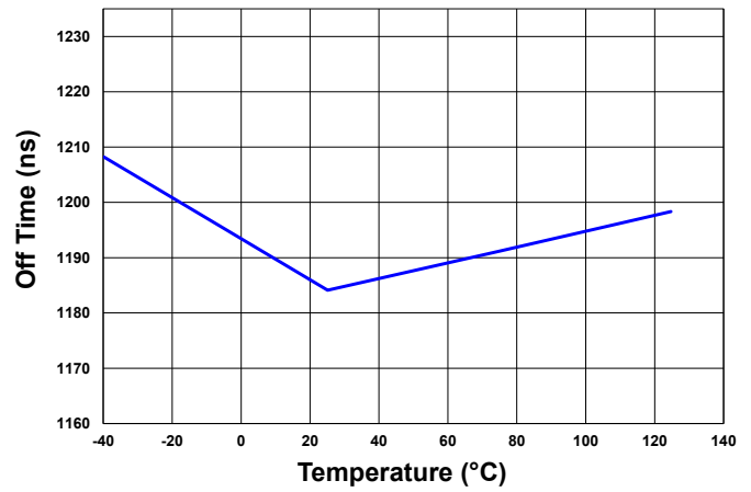
Figure 4-7. OFF Time vs. Temperature
