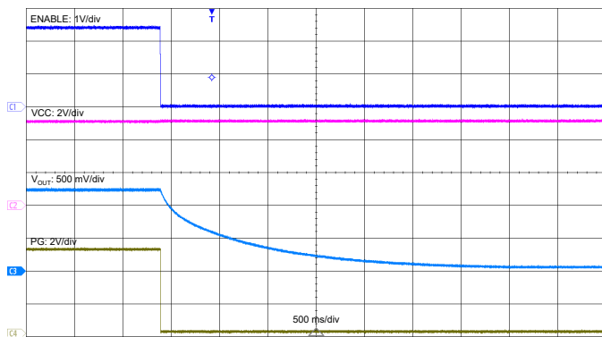
Figure 4-18. Shutdown via EN De-assertion (No Load)
