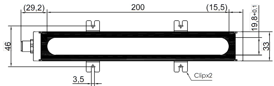
Mounting Diagram_Clip
