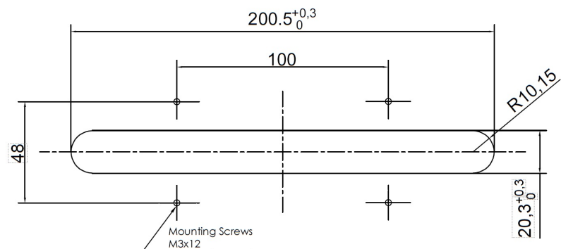
Mounting Diagram_Clip
