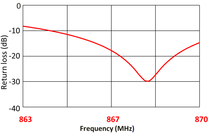
Return Loss
