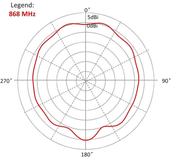
Elevation 2(YZ)
