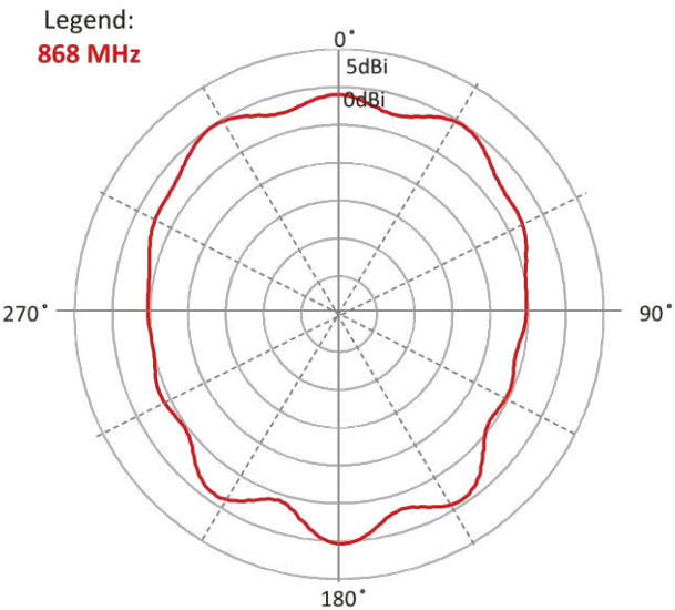
Elevation 1(XZ)
