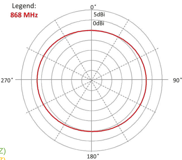
Azimuth(XY)
