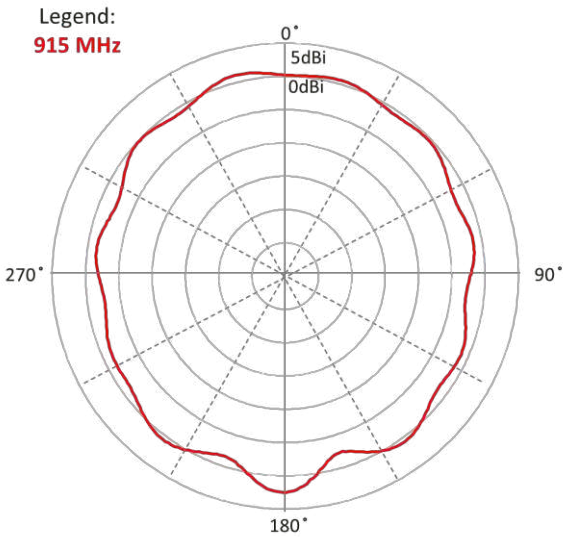
Elevation 2(YZ)
