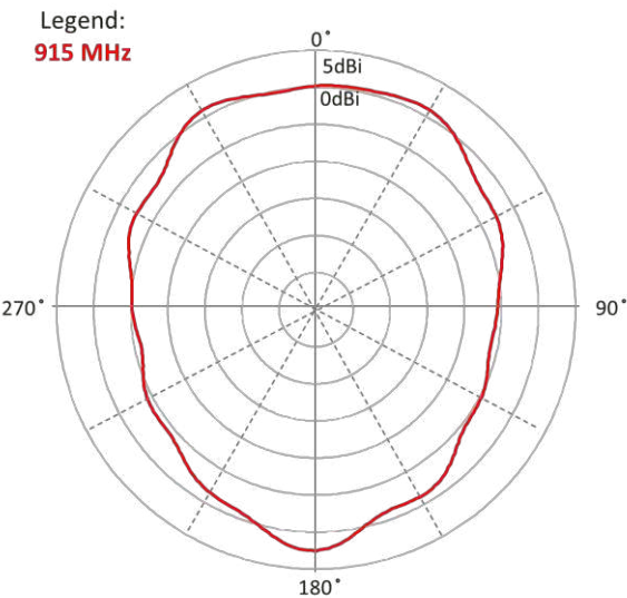
Elevation 1(XZ)
