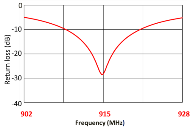
Return Loss
