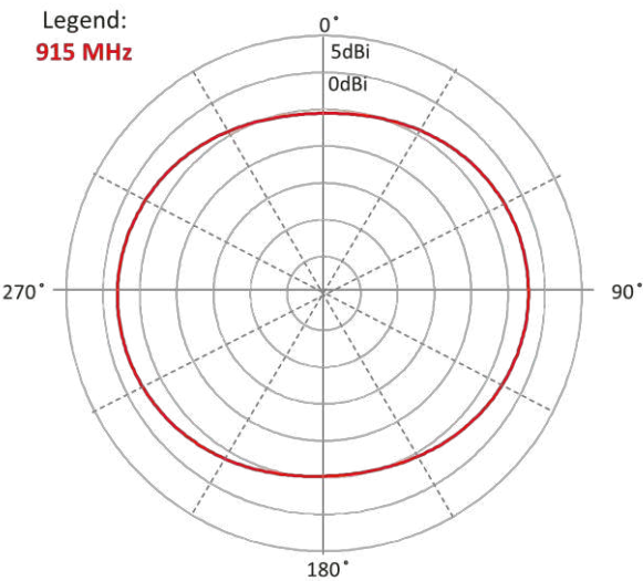
Azimuth(XY)
