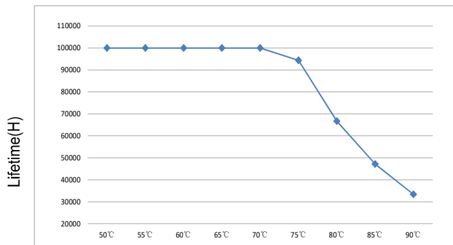
case temperature(Tc)
