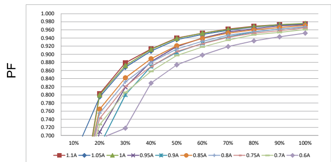
Power factor vs. Load
