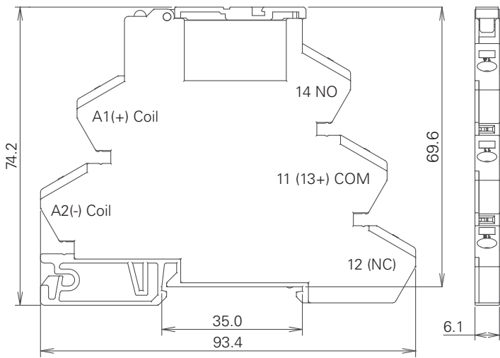
RV8H-S Spring Clamp Terminal (mm)
