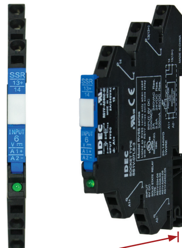
Top view with marking plate
