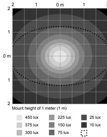
Isolux Pattern
