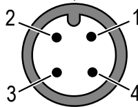
4-pin M12 male quick disconnect
