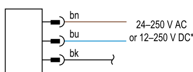
Q453EQ Emitters with quick-disconnect 3-pin Mini male
