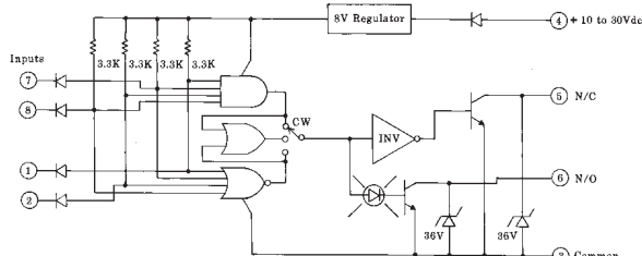
Functional Schematic, MA4G LOGIC Module
