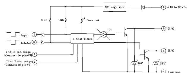
Functional Schematic, MA4-2 ONE-SHOT Module
