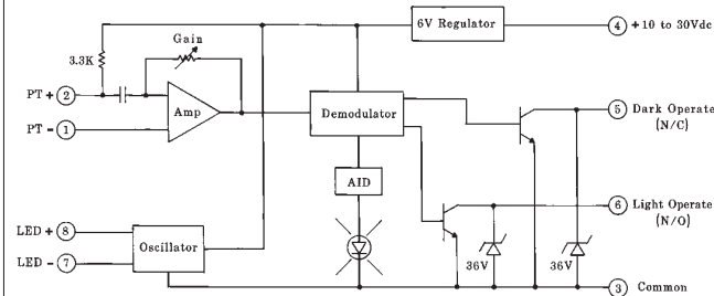
Functional Schematic, MA3-4
