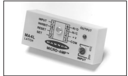
Flip-flop (÷2) logic, MA4L:
