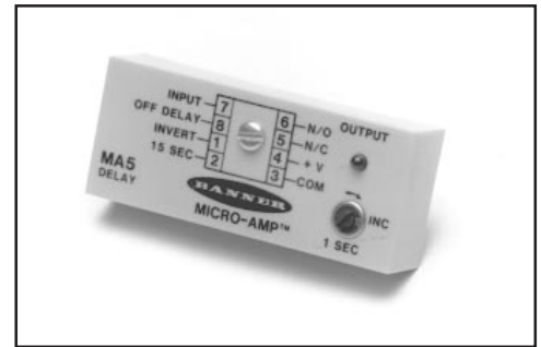
On-delay logic, MA5:
