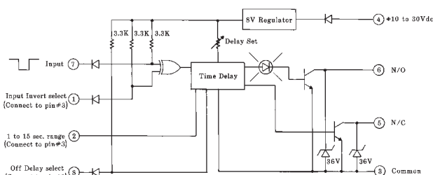
Functional Schematic, MA5 DELAY Module
