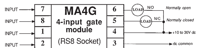
Hookup Diagram, MA4G LOGIC Module
