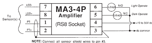
Hookup Diagram, MA3-4P
