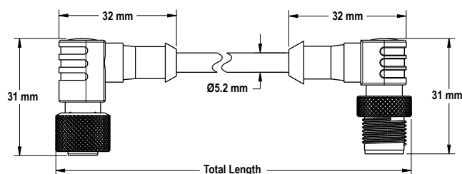
Figure 6. MQDEC..RR dimensions
