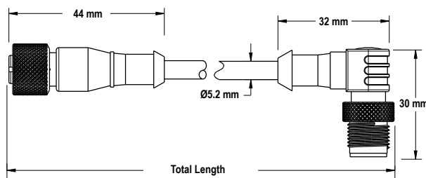
Figure 5. MQDEC..RS dimensions
