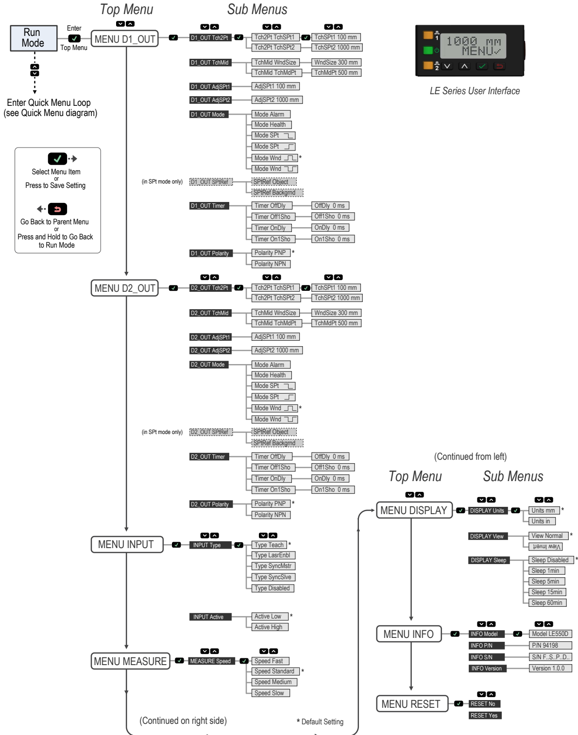
LE550 Sensor Menu Map
