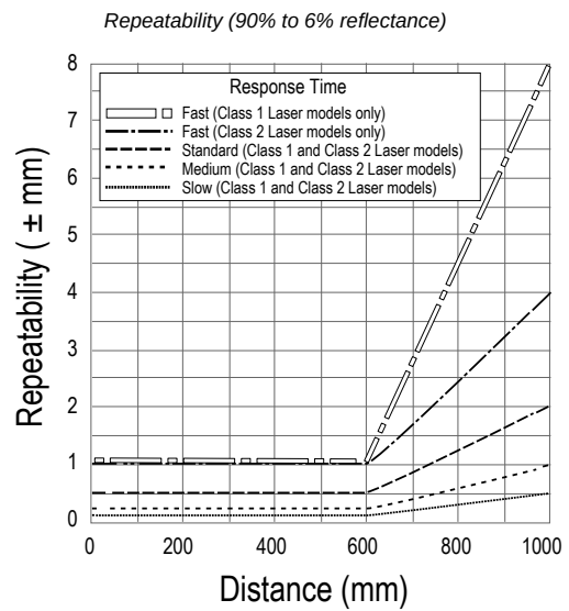
LE550 Dual Discrete Models
