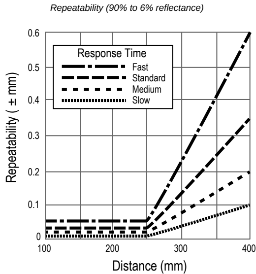
LE250 Dual Discrete Models
