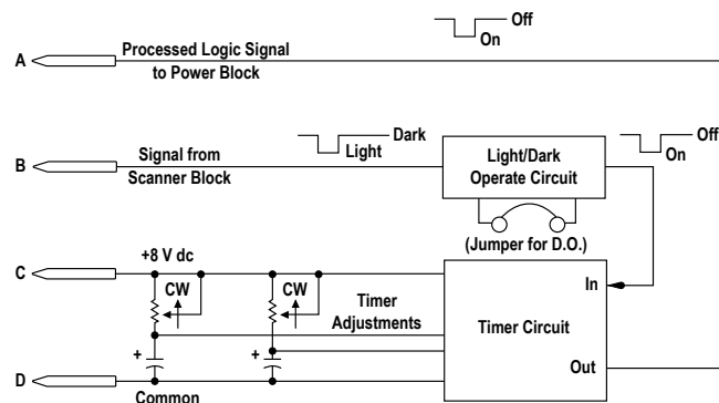
Figure 1. Functional Schematic
