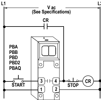
Figure 10. Wiring in Series with Contacts or Switches
