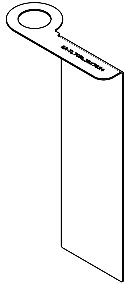
ISOMETRIC VIEW SCALE 1:2
