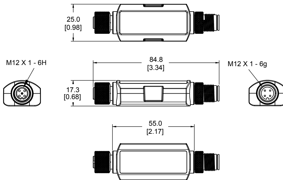
Figure 1. LC25 dimensions
