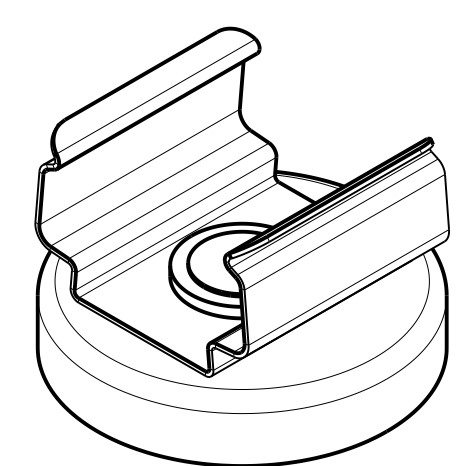
ISOMETRIC VIEW SCALE 3:2
