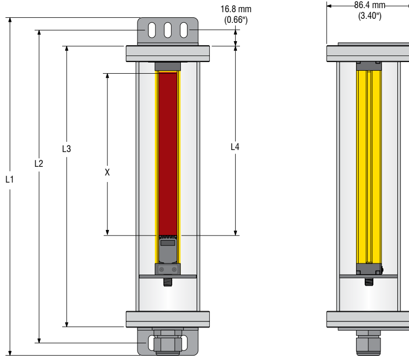
Figure 3. Enclosure/EZ-SCREEN dimensions
