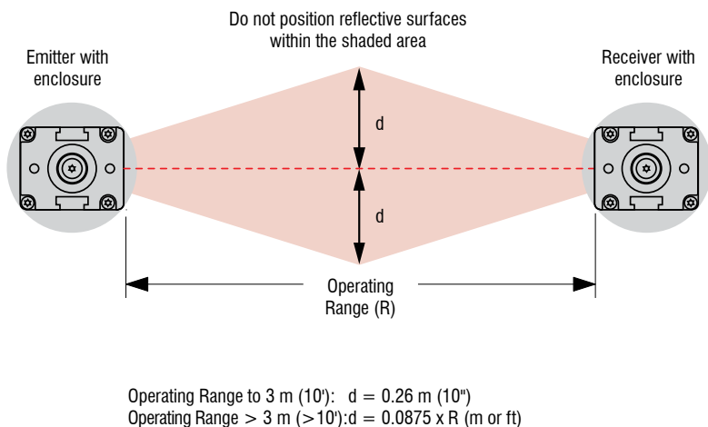
Figure 2. Adjacent reflective surfaces
