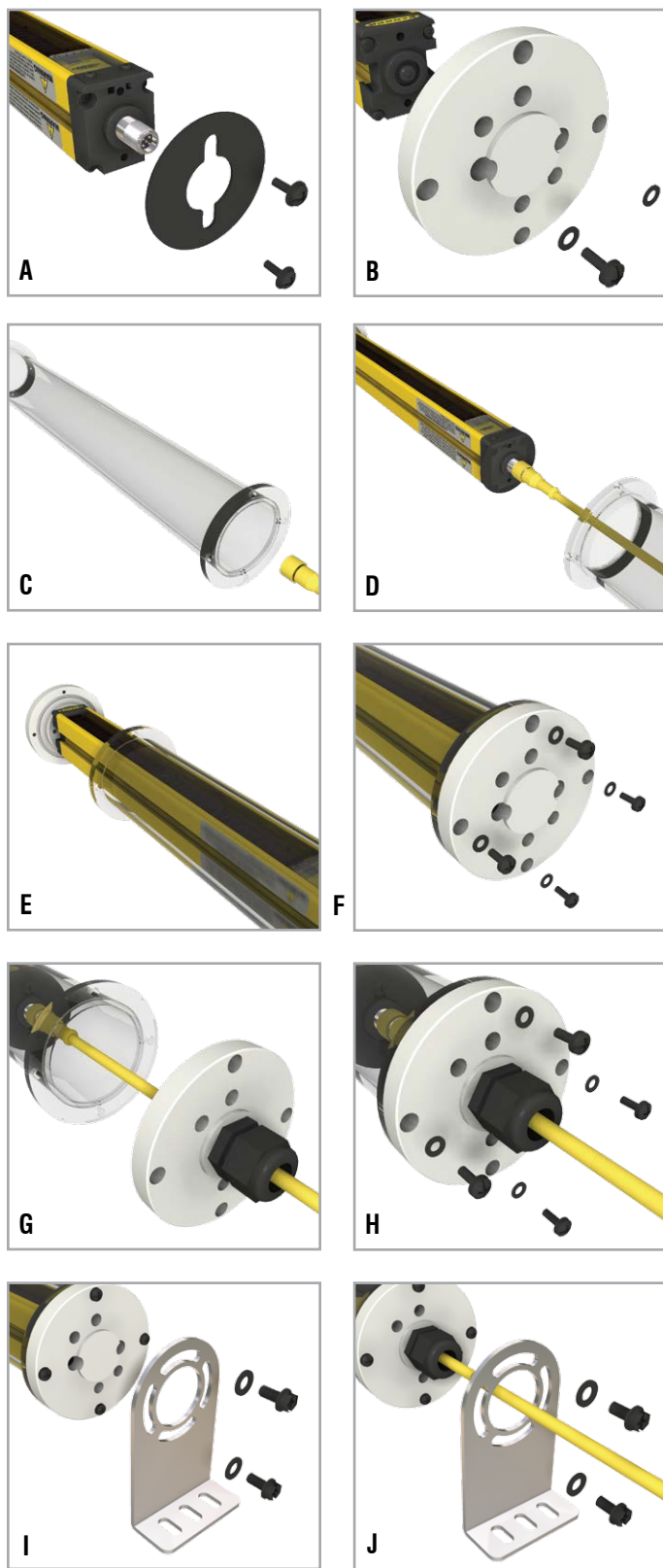
Figure 4. EZA-TE Series Tubular Enclosure assembly steps
