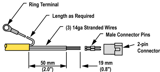
Figure 3. Assembly of the Molex connector
