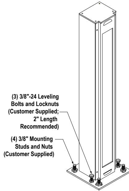
Figure 2. Level the heated enclosure
