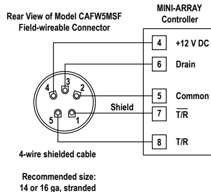
Figure 4. MINI-ARRAY sensor cable wiring to the field-wireable connector
