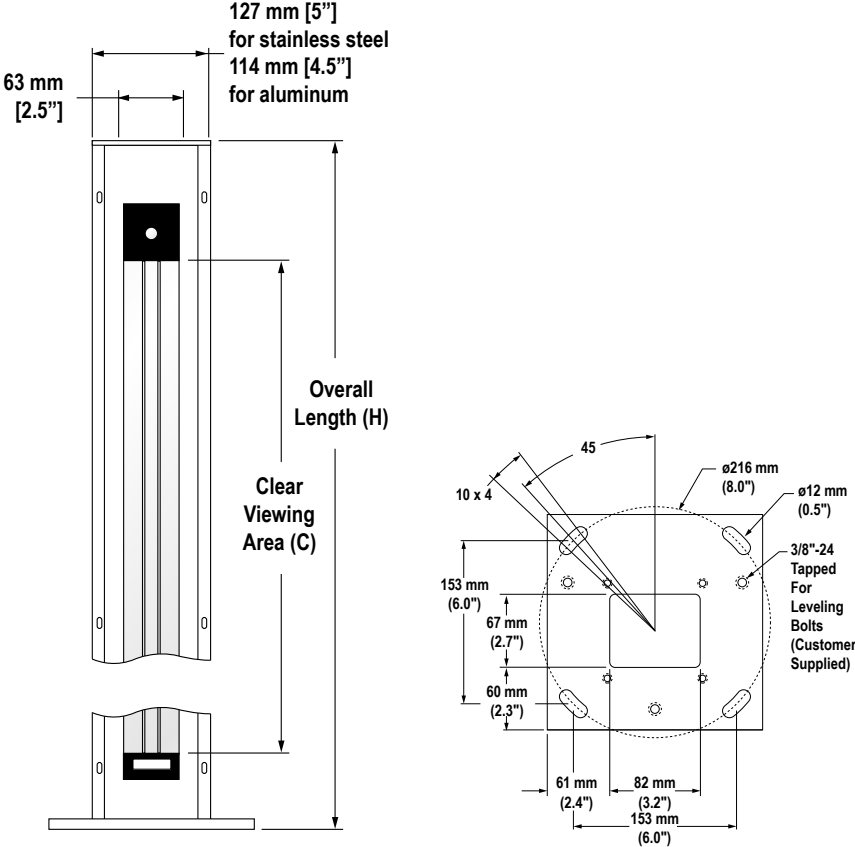
Figure 5. Dimensions
