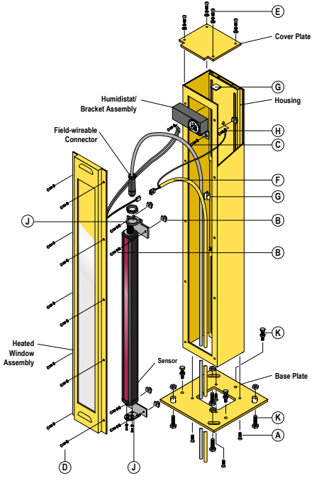
Figure 1. Exploded view of the assembly
