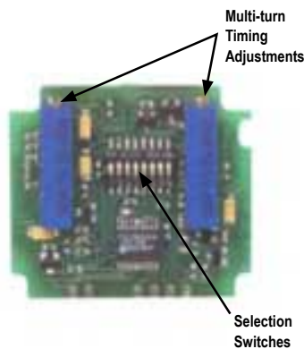
Figure 1. 45LM58 Features
