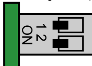
DIP switch settings for dual- and single-channel (switch 1 and 2 are ON)
