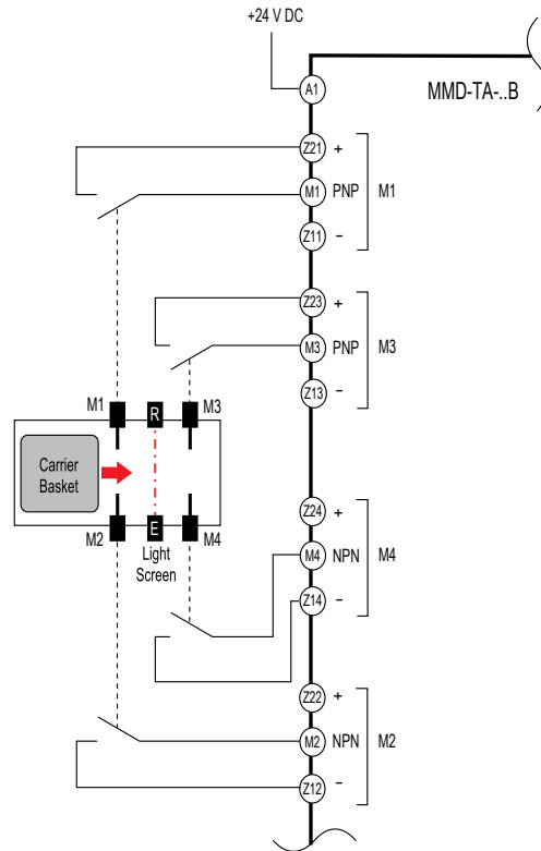
Figure 9. Four Limit Switches as M1, M2, M3, and M4
