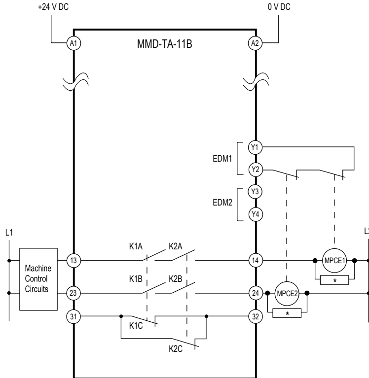
Figure 34. Generic machine interface wiring, model MMD-TA-11B: MPCE with 1-channel EDM
