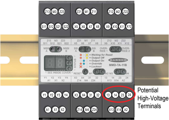
Figure 5. MMD-TA-11B terminal connection locations
