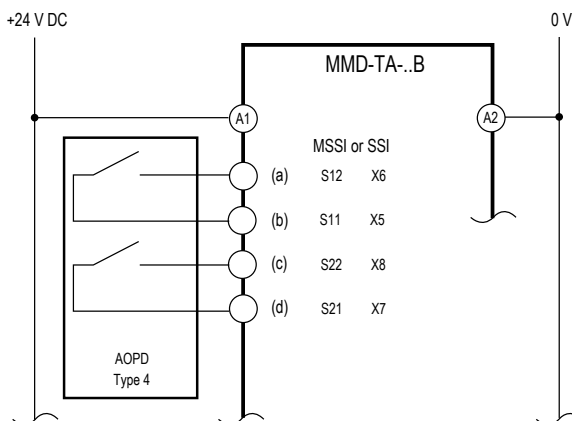
Figure 22. MSSl and SSl Category 4 interfacing: category 4 safeguarding device with relay outputs (for example, MINI-SCREEN or AOPD Type 4 per IEC 61496-1/-2)
