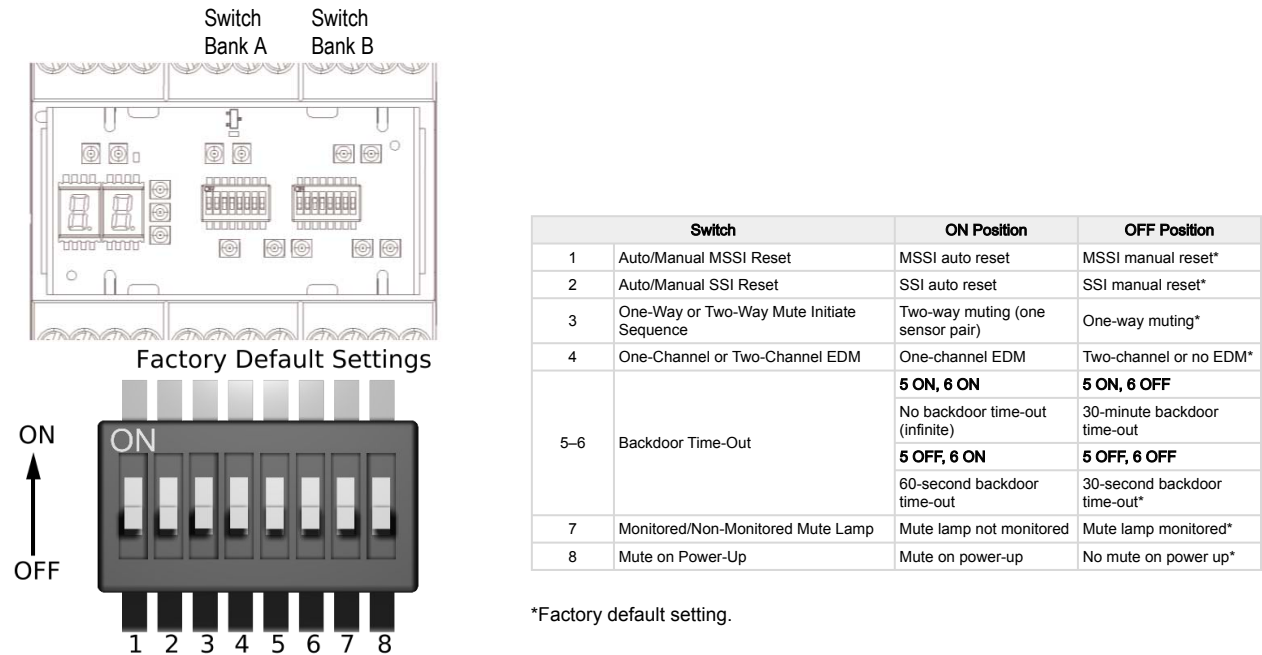
Figure 4. Muting Module manual configuration parameters
