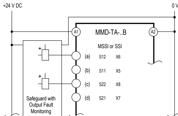
Figure 19. MSSl and SSl Category 3 interfacing: Category 3 safeguarding device with output fault monitoring (for example, type 3 area scanner AOPDDR per IEC 61496-1/-3)
