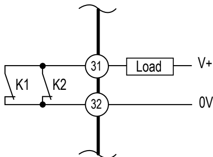
Figure 13. AUX output wiring — MMD-TA-11B
