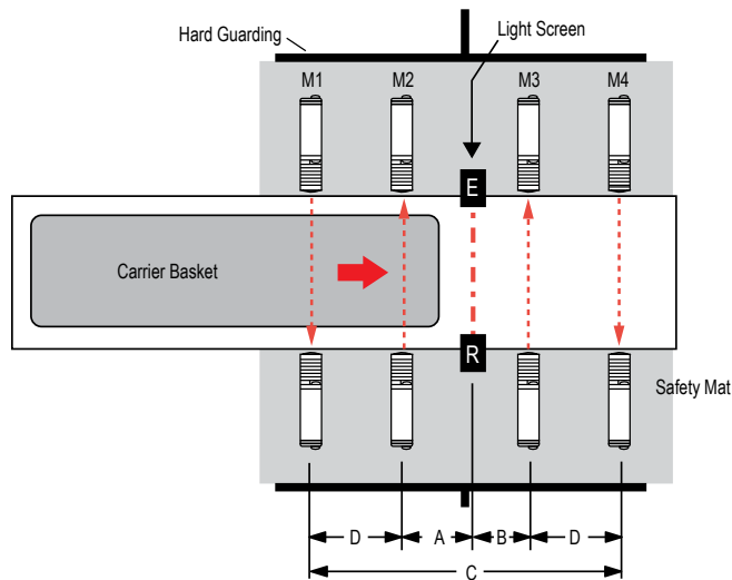
Figure 40. An entry/exit system using four photoelectric sensors as M1, M2, M3, and M4
