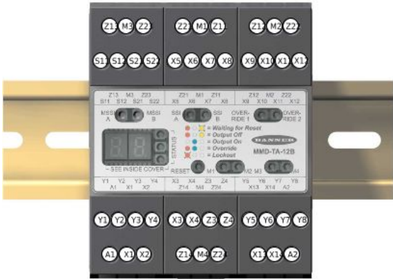
Figure 6. MMD-TA-12B terminal connection locations
