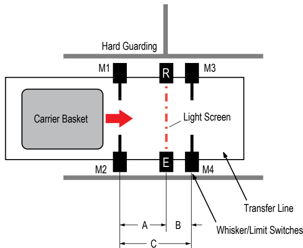
Figure 39. Entry/exit system using 4 whisker/limit switches as muting devices
