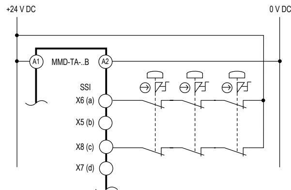
Figure 24. SSI Category 3 interfacing: positive-opening E-stop switch(es)
