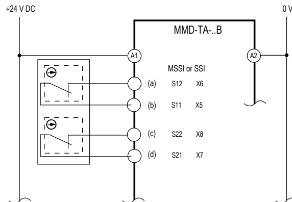
Figure 21. MSSl and SSl Category 4 interfacing: category 4 safeguarding device with output fault monitoring (for example, EZ-SCREEN or AOPD Type 4 per IEC 61496- 1/-2)
