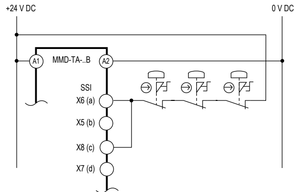
Figure 23. SSI Category 2 interfacing: positive-opening E-stop switch(es)
