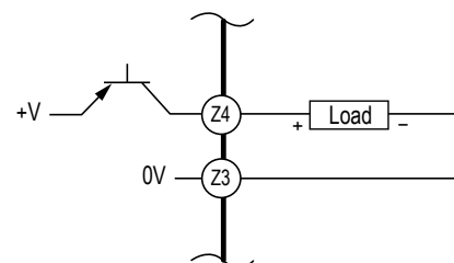
Figure 14. AUX output wiring — MMD-TA-12B
