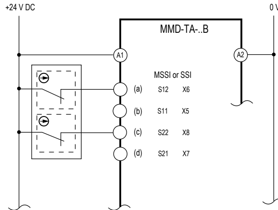
Figure 19. MSSl and SSl Category 3 interfacing: Category 3 safeguarding device with output fault monitoring (for example, type 3 area scanner AOPDDR per IEC 61496-1/-3)
