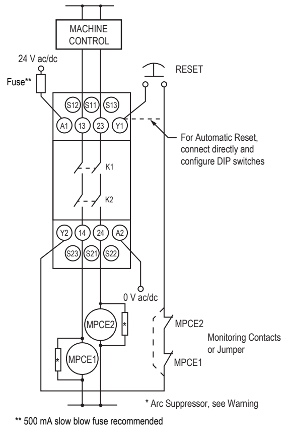
Wiring to the guarded machine
