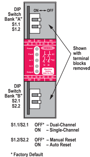
DIP switch configuration settings for reset mode and single- or dual-channel operation
