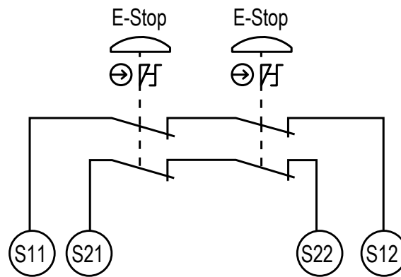
Series connection of multiple e-stop switches
