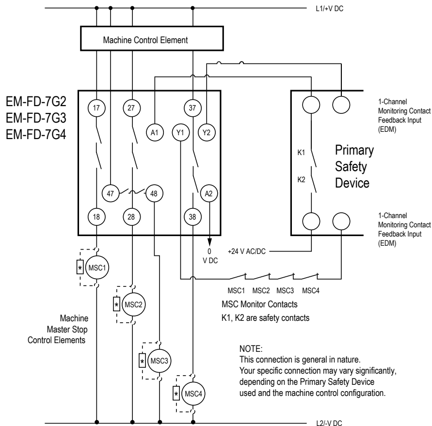
Generalized EM-FD-7G Series Connection Diagram
