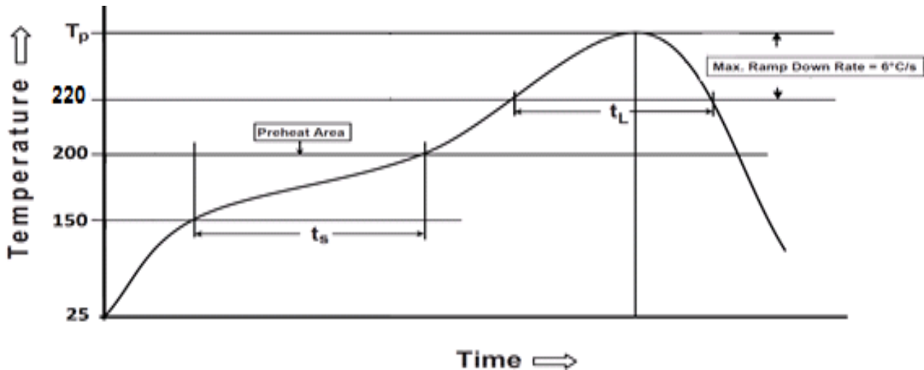
Figure 23: Temperature profile
