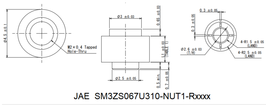
Figure 13: Mounting information for the Sona TI351 M.2 2230 module and recommended layout pattern for the stand-off
