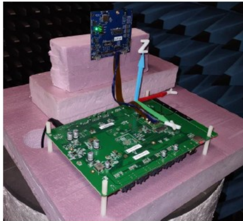
Figure 24: Sona TI351 Radiated Performance Measurement Setup
