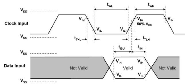
Figure 6: SDIO bus Input timing- High Speed mode (1.8V)
