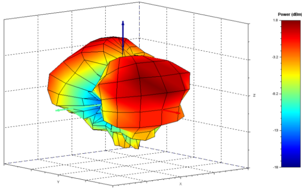
Figure 33: Sona TI351 Theta and Phi Polarization Radiated Patterns at 5500 MHz
