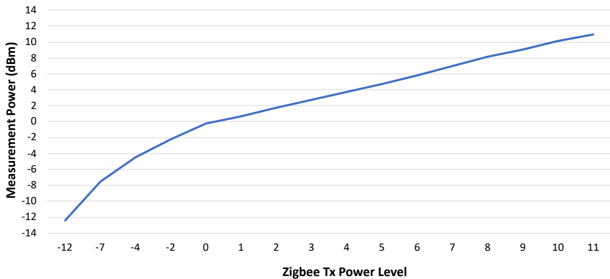
Figure 49-50. Zigbee Transmit Power vs. Power Level
