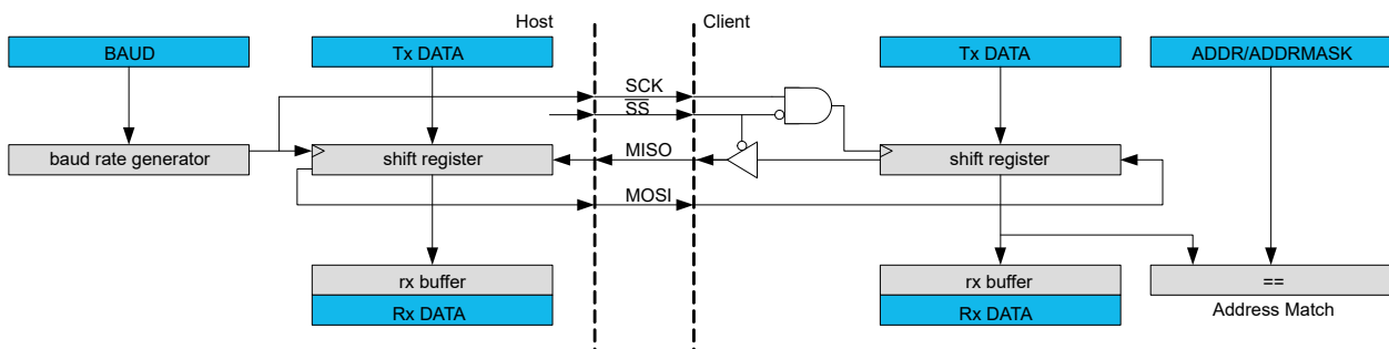
Figure 34-1. Full-Duplex SPI Host Client Interconnection
