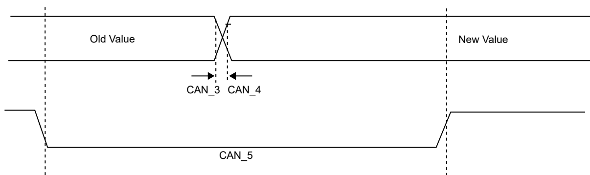
Figure 49-26. CANx Module AC Timing Diagram
