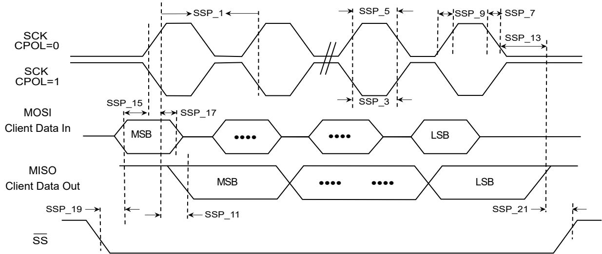
Figure 49-21. SPI Client Module CPHA = 1 Timing Diagrams
