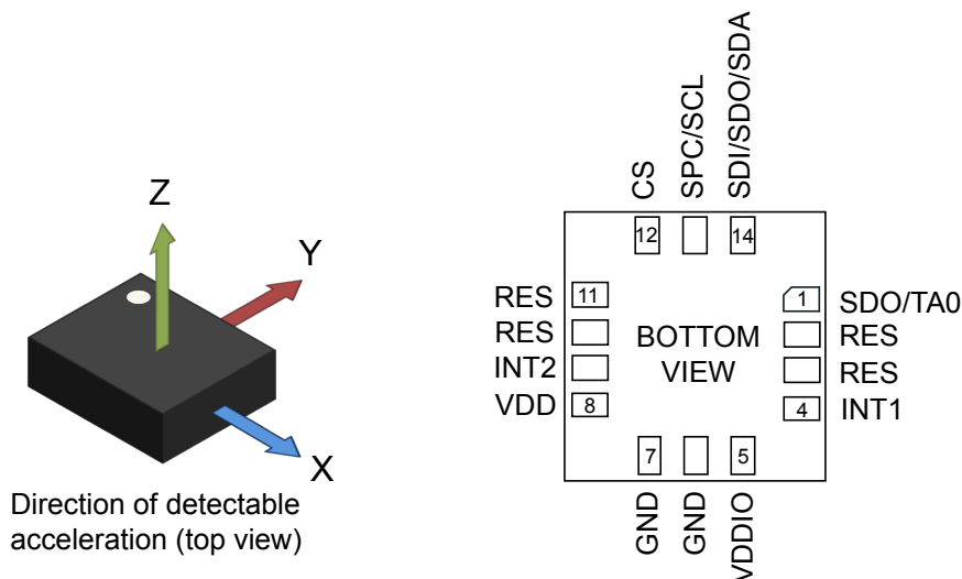
Figure 1. Pin connections
