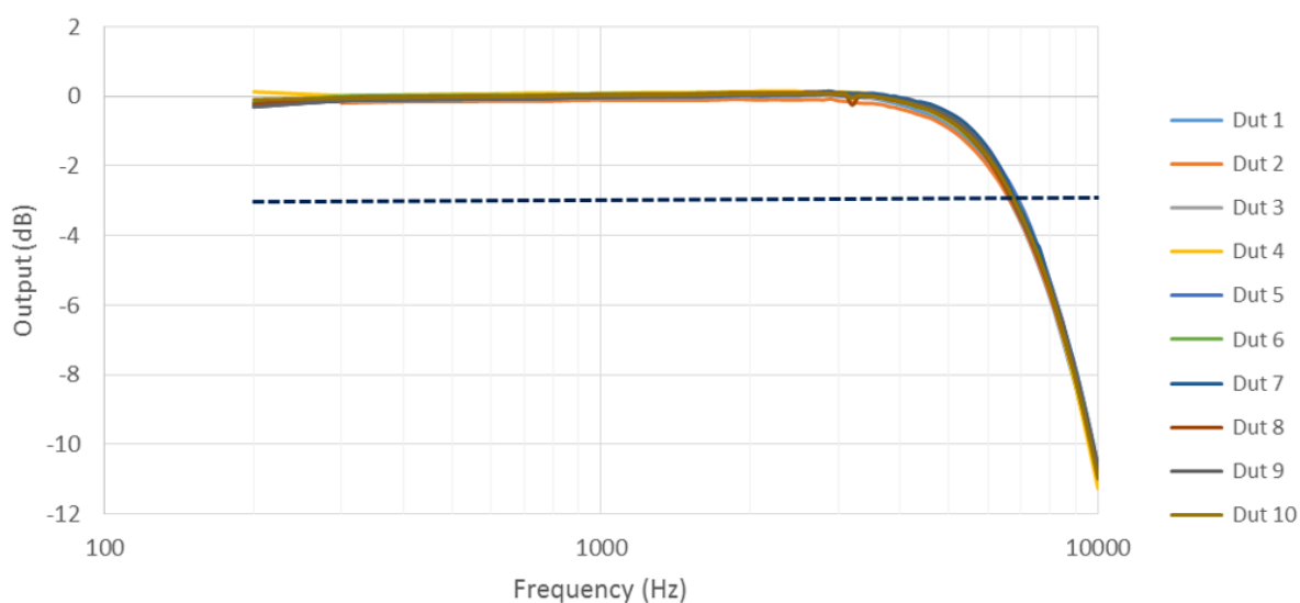
Figure 16. Frequency response - Y-axis
