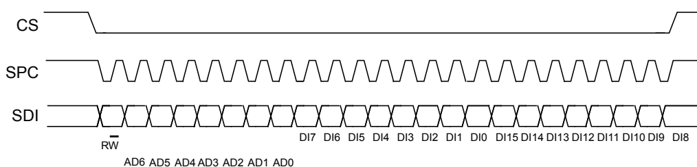
Figure 7. Multiple byte SPI write protocol (2-byte example) (in mode 3)
