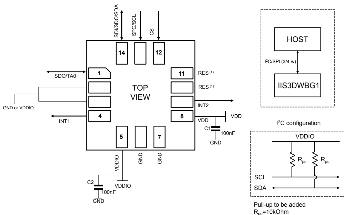
Figure 20. IIS3DWBG1 electrical connections
