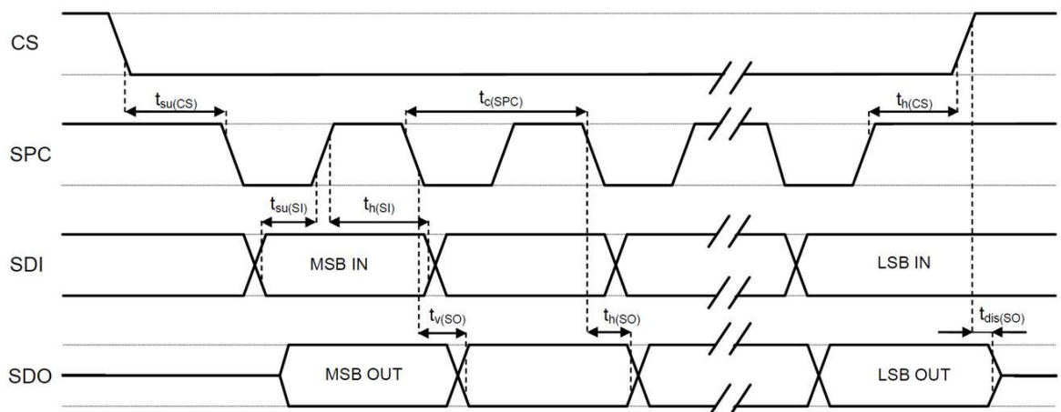
Figure 2. SPI target timing diagram
