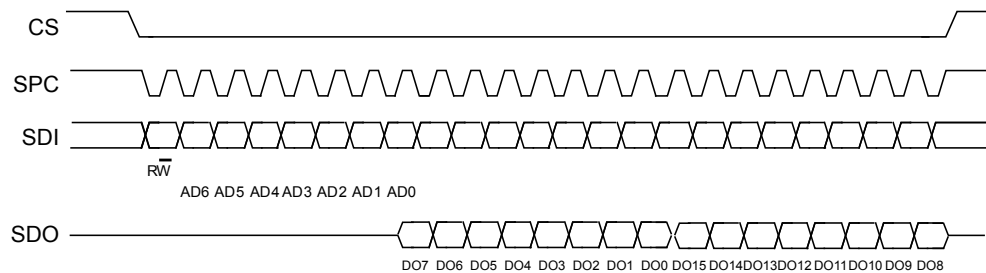
Figure 5. Multiple byte SPI read protocol (2-byte example) (in mode 3)
