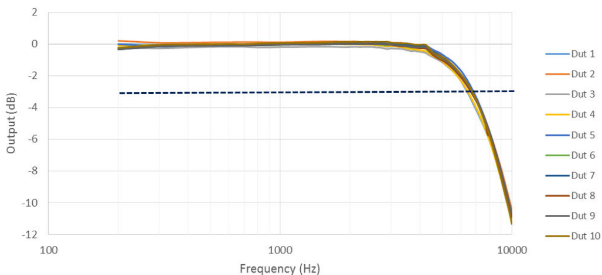
Figure 15. Frequency response - X-axis
