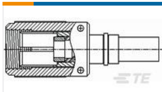
TE Part #601154-000 D-621-0011
