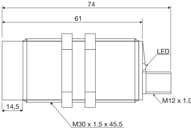
Fig. 9 Plug CA30CAN...M1IO
