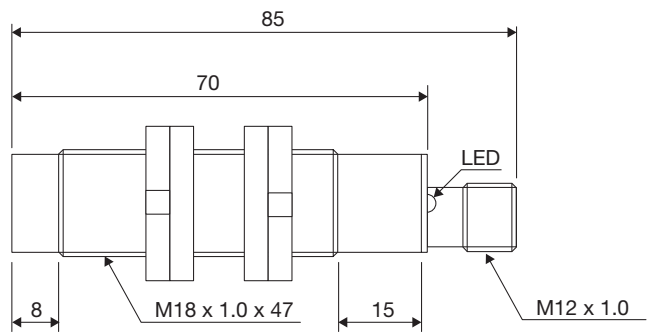
Fig. 9 Plug CA18CAN...M1IO
