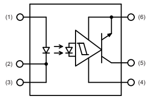
Internal circuit
