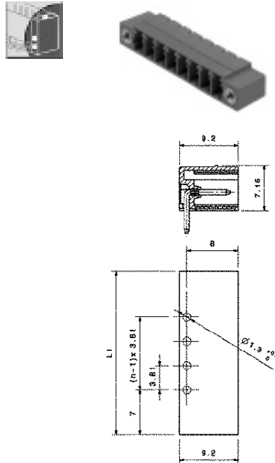
Pin headers SL 3.81/90F
