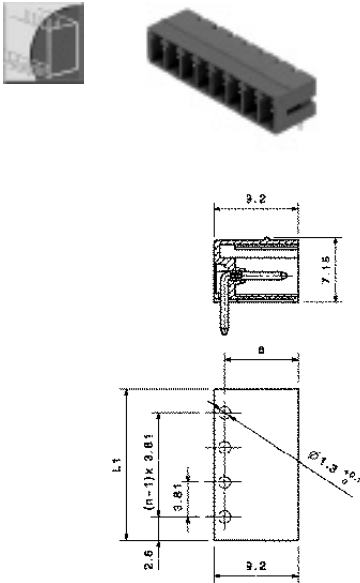
Pin headers SL 3.81/90G
