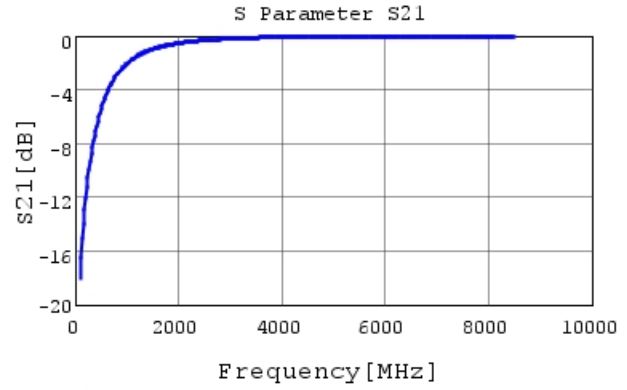
GCQ1555C1H2R0CB01 S21 DCOV, 25degC
