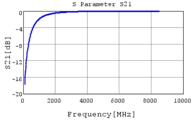
GCQ1555C1H2R1BB01 S21 DCOV, 25degC
