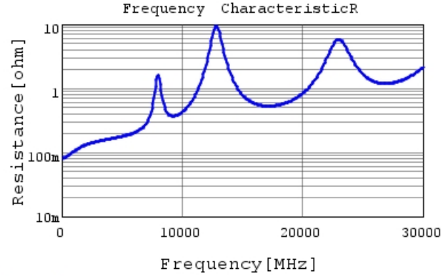
GJM0335C1E120FB01 R DCOV, 25degC
