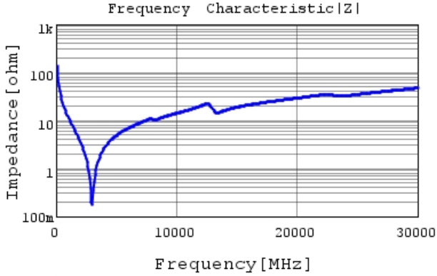
GJM0335C1E120FB01 |Z| DCOV, 25degC
