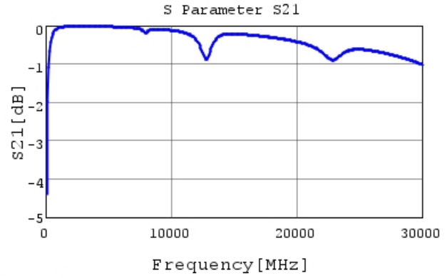
GJM0335C1E120FB01 S21 DCOV, 25degC
