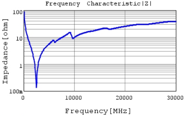
GJM0335C1E180FB01 |Z| DCOV, 25degC
