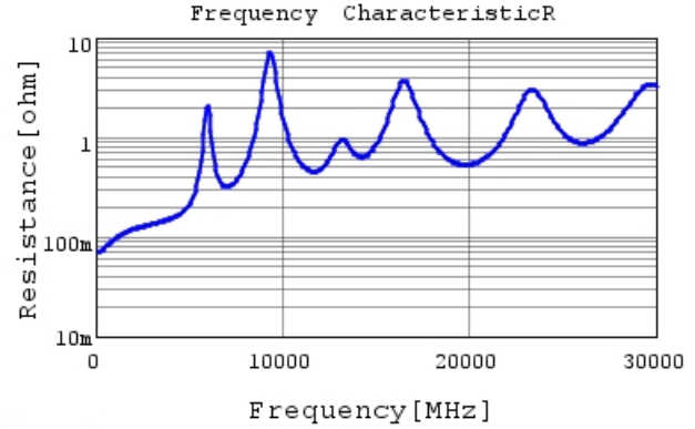
GJM0335C1E180FB01 R DCOV, 25degC
