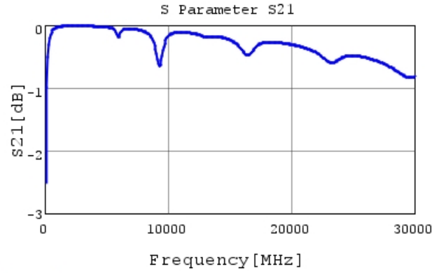
GJM0335C1E180FB01 S21 DCOV, 25degC
