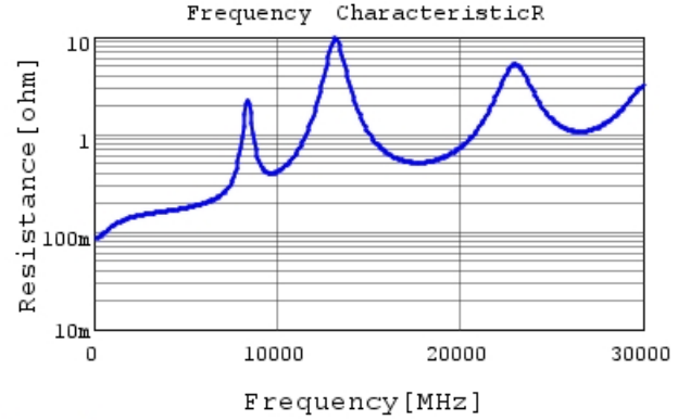
GJM0335C1E100FB01 R DCOV, 25degC
