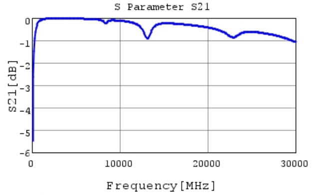
GJM0335C1E100FB01 S21 DCOV, 25degC
