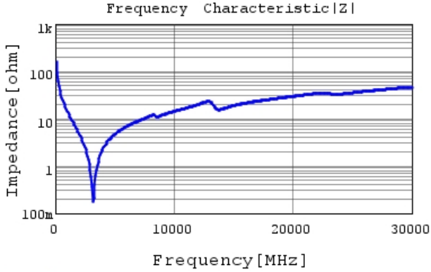
GJM0335C1E100FB01 |Z| DCOV, 25degC
