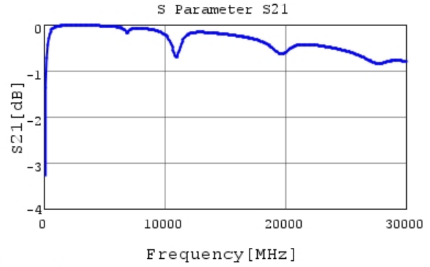
GJM0335C1E150FB01 S21 DCOV, 25degC
