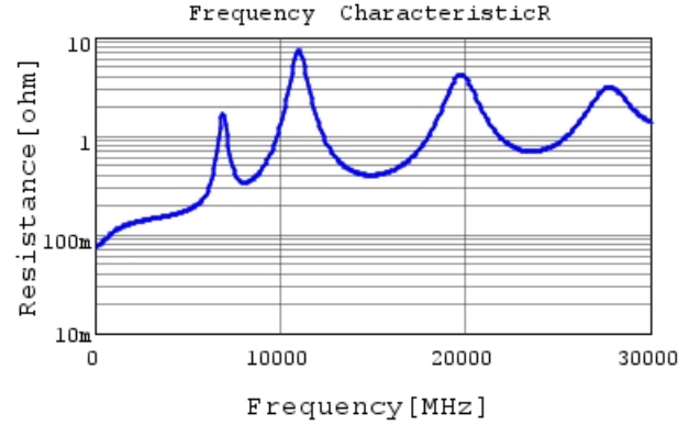
GJM0335C1E150FB01 R DCOV, 25degC
