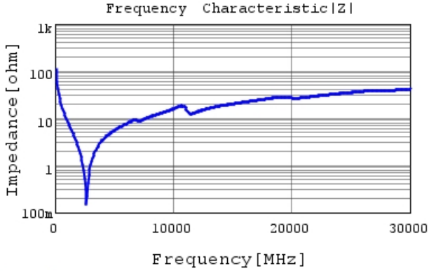
GJM0335C1E150FB01 |Z| DCOV, 25degC
