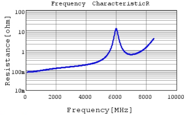
GCQ1555C1H120GB01 R DC0V, 25degC
