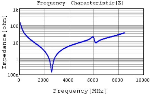
GCQ1555C1H120GB01 |Z| DC0V, 25degC
