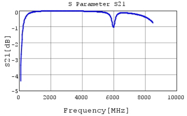
GCQ1555C1H120GB01 S21 DCOV, 25degC
