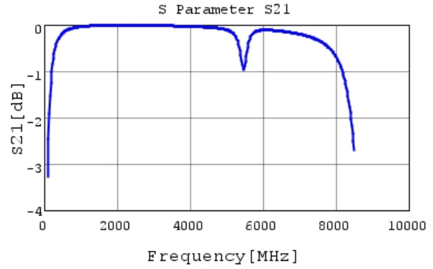
GCQ1555C1H150FB01 S21 DCOV, 25degC
