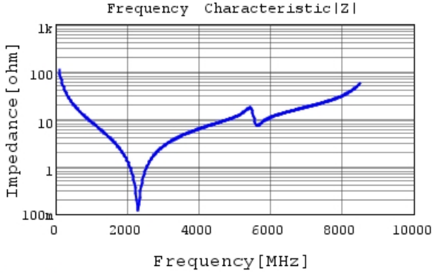
GCQ1555C1H150FB01 |Z| DC0V, 25degC
