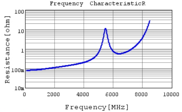
GCQ1555C1H150FB01 R DC0V, 25degC
