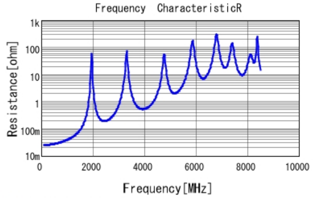
■ GQM22M5C2H680JB01 R DC0V, 25degC
