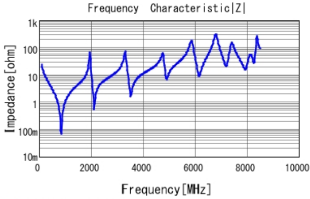
■ GQM22M5C2H680JB01 |Z| DC0V, 25degC
